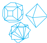
\text{CaF}_2
